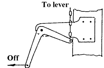
Crank fitted at base of post to change motion from horizontal to vertical
